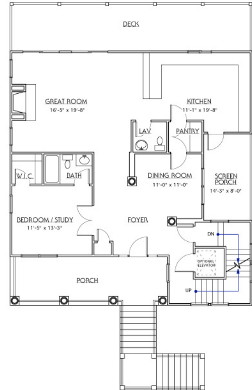
MAIN FLOOR PLAN 1357 SQ. FT. HEATED
