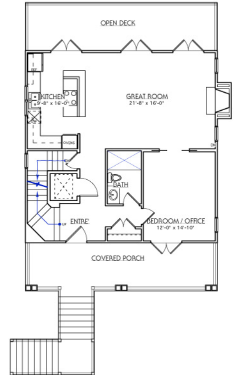
MAIN FLOOR PLAN 1024 SQ. FT. HEATED
