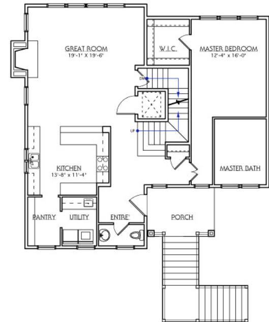
MAIN FLOOR PLAN 1360 SQ. FT. HEATED
