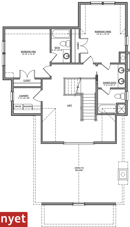
Second Floor Plan 981 heated square feet
