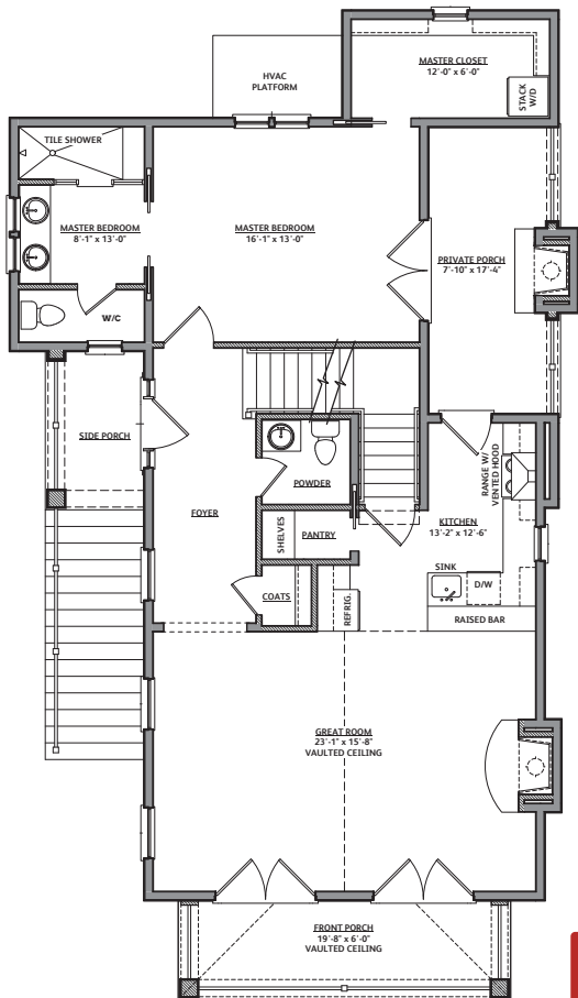
First Floor Plan 1211 heated square feet
