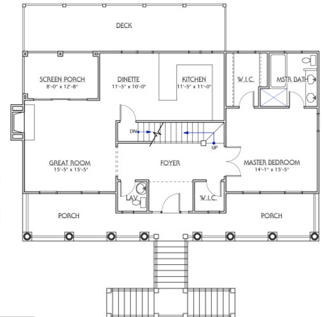
MAIN FLOOR PLAN 1160 SQ. FT. HEATED
