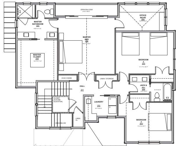
Second Floor Plan 1380 heated square feet
