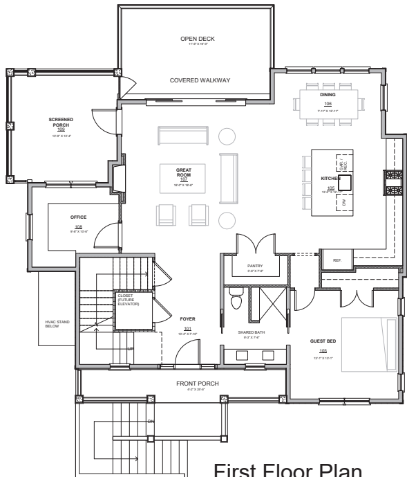
First Floor Plan 1390 heated square feet
